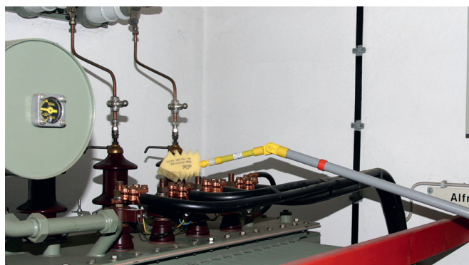
Damp cleaning of a transformer using the FRS ZK MS damp cleaning kit.
