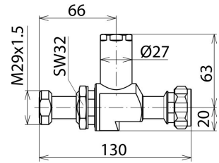
Dimension drawing DGA L4 7 16 MFA
