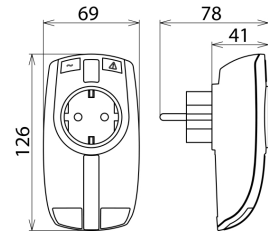
Dimension drawing DPRO 230 NT
