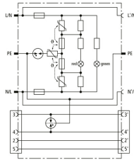
Basic circuit diagram DPRO 230 NT
