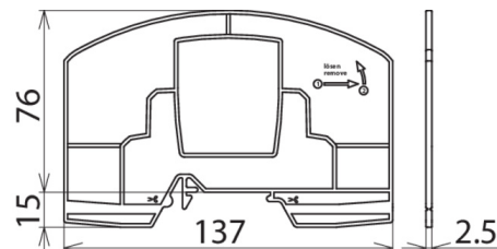
Dimension drawing of the partition
