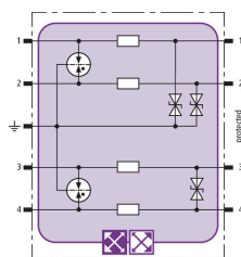
Basic circuit diagram BXT ML4 BE BD 24
