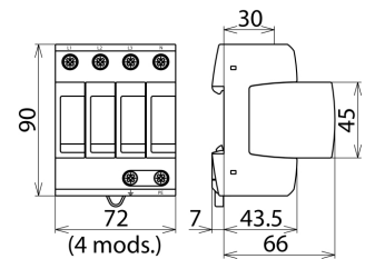
Dimension drawing DG M TT 385
