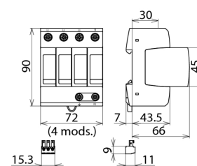
Dimension drawing DG M TNS 150 FM
