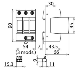
Dimension drawing DG M TNC 150 FM
