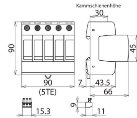
Dimension drawing DG M PV2 SCI SN1868
