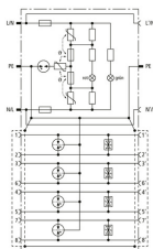
Basic circuit diagram DPRO 230 LAN100
